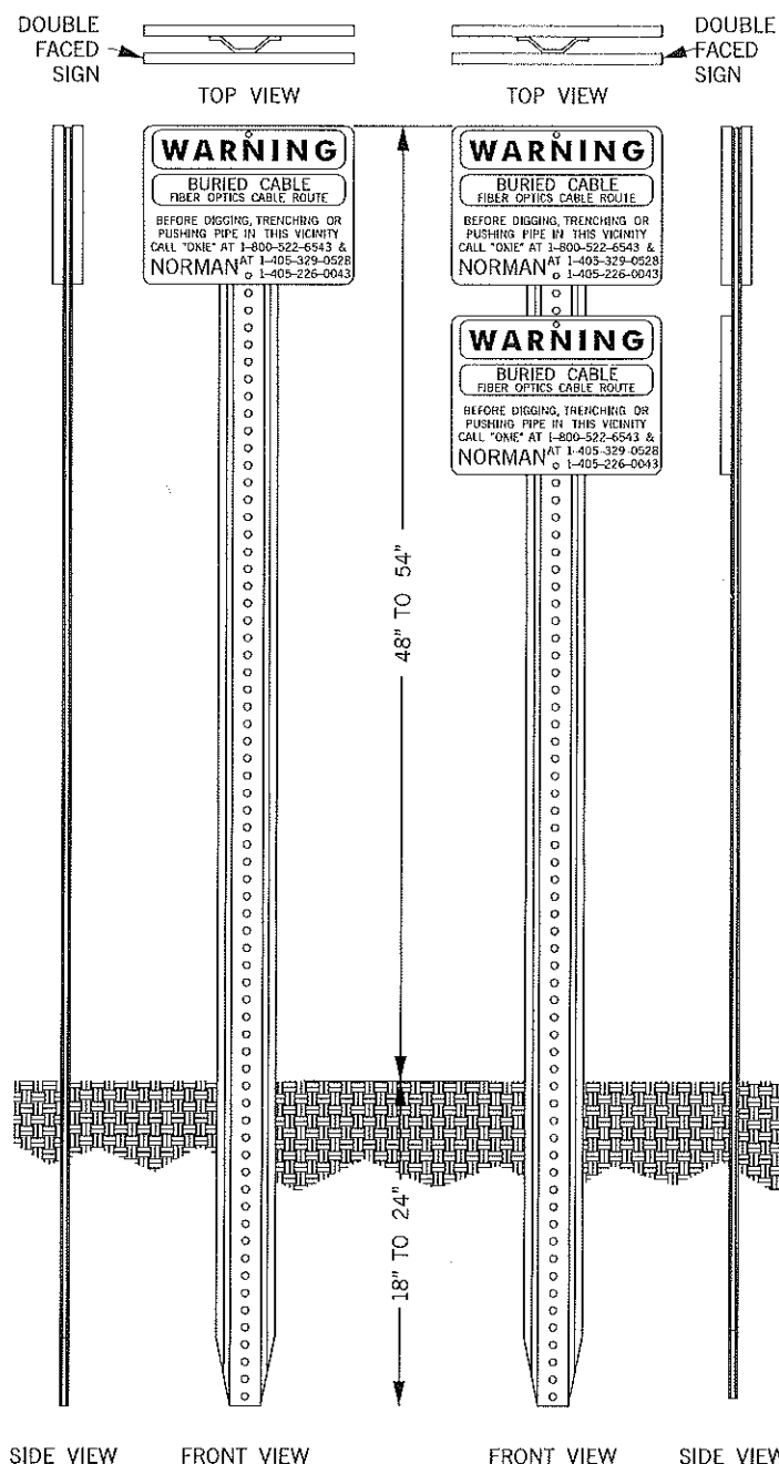
TYPE "A" FOR PLACEMENT ALONG FIBER ROUTE TYPICAL SIGN PLACEMENT TYPE "B" FOR PLACEMENT AT GROUND BOX LOCATIONS TYPICAL SIGN PLACEMENT
